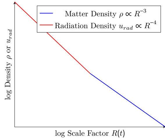
Figure 22.1: Density as a function of scale factor, showing the difference between matter and radiation domination. It can be shown that a = \frac{R}{R_0} = \frac{1}{3500} and \frac{t}{t_0} = \frac{1}{2 \times 10^5 \text{ unit}} .
