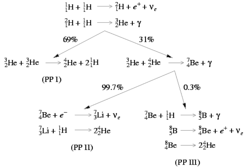
Figure 4.1: https://burro.cwru.edu/academics/Astr221/StarPhys/ppchain.html
